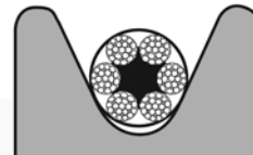
Sheave groove too narrow
